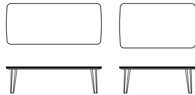
7AND101 Top in marmo / Marble top Base in legno / Wooden base L255 P110 H71,5 7AND103 Top in marmo / Marble top Base in legno / Wooden base L205 P100 H71,5
