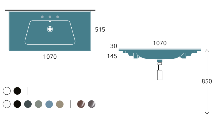
Bloom 105 art. BM105L
