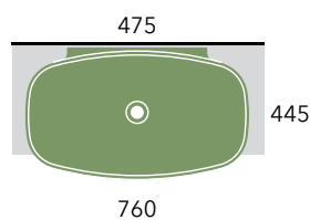
NudaSlim 75 art. ND75L
