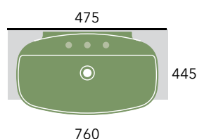
NudaSlim 75 art. ND75PR
