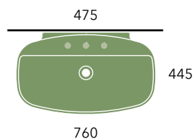
NudaSlim 75 art. ND75PR
