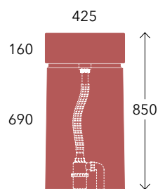
Twin Column art. 5050/COLC + 5050/42C
